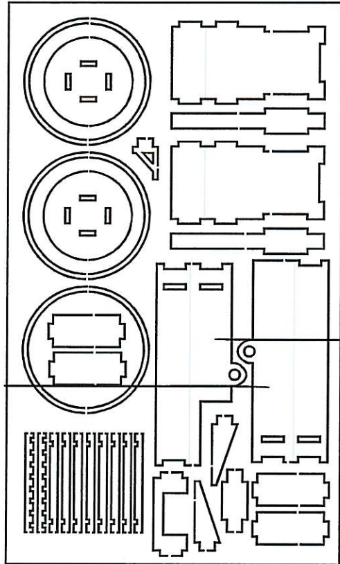
WATER WHEEL SHEET 1
