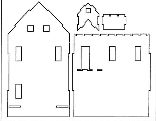
WALL SHEET 2
